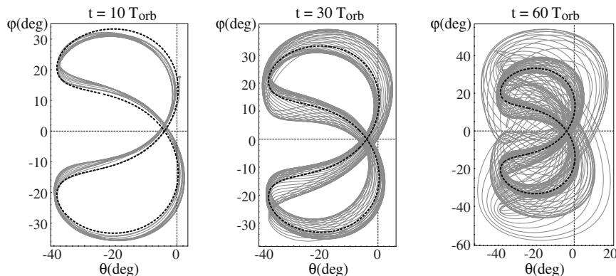
Fig. 7 Failure of the TDAS control method for the case of \varepsilon = 1.5 and i = 40^\circ . Libration motion after 10, 30, and 60 orbital periods. Control parameters are k_1 = 0.2 and k_2 = 1.2 . The dashed line represents the corresponding periodic motion.
