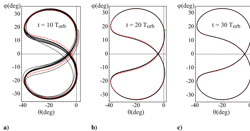
Fig. 9 Success of the ETDAS control method for the case of \varepsilon = 1.5 and i = 40^\circ deg. Controlled librational motion after 10, 20, and 30 orbital periods. Control parameters are k_1 = k_2 = -0.2 and R_1 = R_2 = 0.9 . The dashed line stands for the corresponding periodic motion. In b) and c), only the libration during the two last orbital periods is represented.
