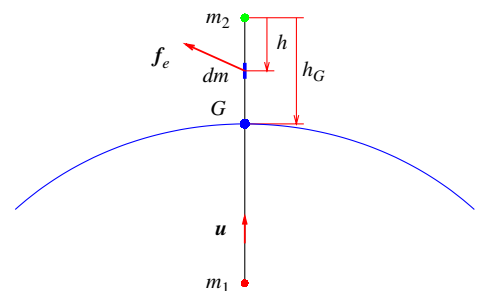
Fig. 1 System mass geometry.
