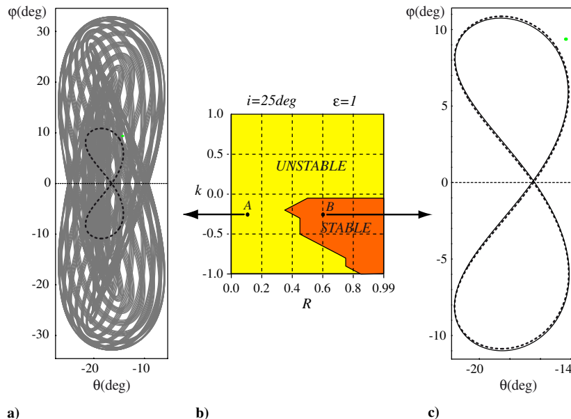
Fig. 11 Two examples of the different efficacies of the ETDAS method in both regions of the stability domains when \varepsilon = 1 and i = 25^\circ deg: a) unstable control for R = 0.1 and k = -0.25 , b) control domains in the parametric plane ( R , k ), and c) stable control for R = 0.6 and k = -0.25 .
