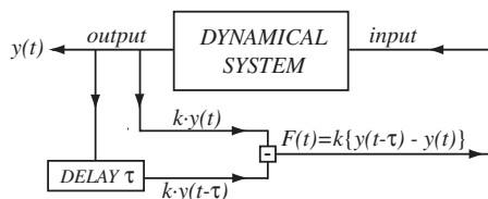
Fig. 6 Block diagram of the TDAS control method.
